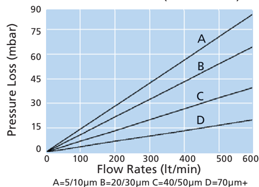
Flow Rates For Water (40" Element)
